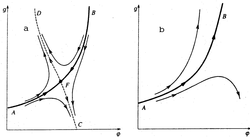
Figure 2: Flow diagram in the (g, \varphi) plane: (a) in the case of existence of the fixed point F on the critical surface AB , (b) in the case of its absence.
